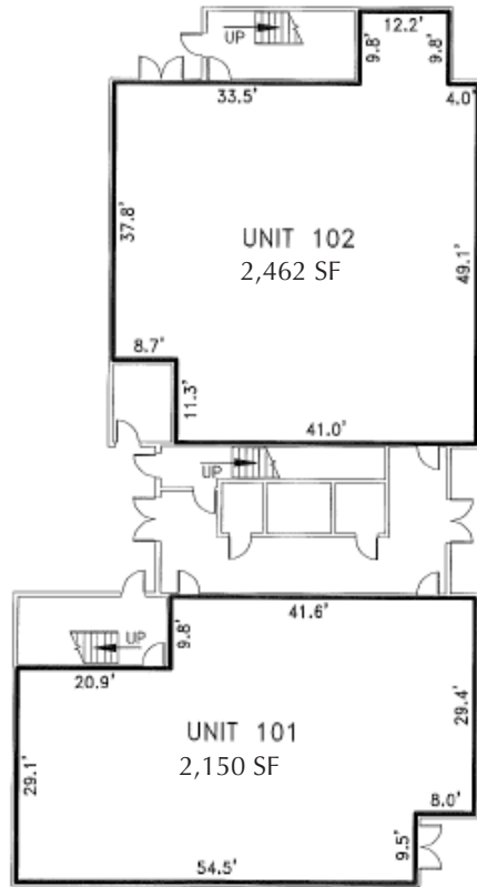
First Floor Layout
